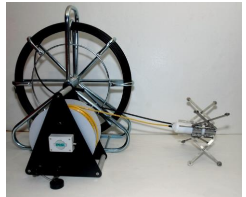
TEL-902-000: adjustable stainless steel horizontal centering device (for ASPO 50 option)
