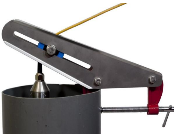
↑ TEL-904-000: pulley assembly (to be fixed at the mouth of the well)
